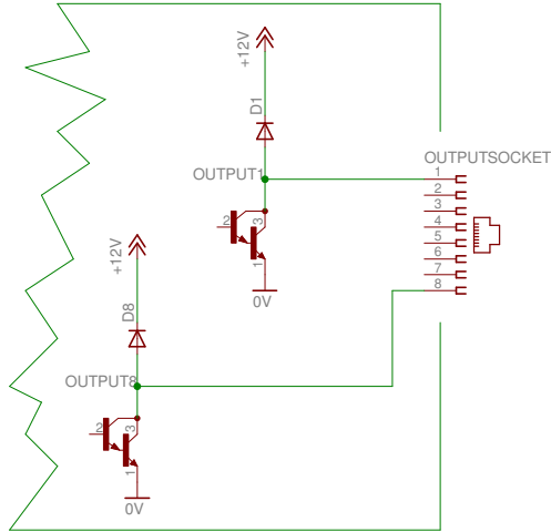
Transistor output circuitry on Ruscool 64 Output PCB
